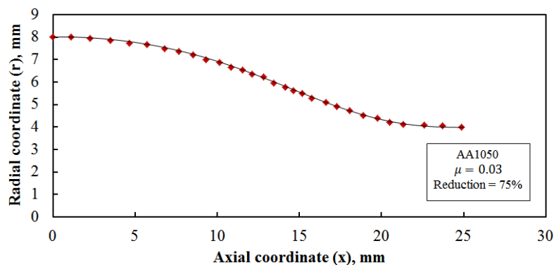
Fig. 3. Optimized die shape predicted by the algorithm
